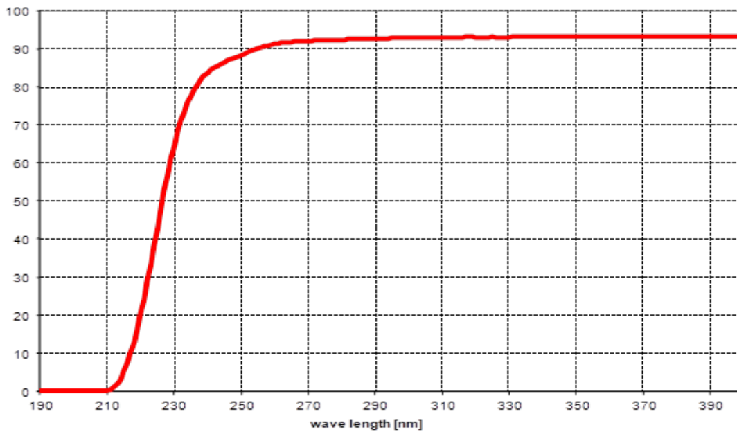
Transmission curve RQ 235
